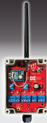
Wireless Max Wiegand Converter 1 mile range
